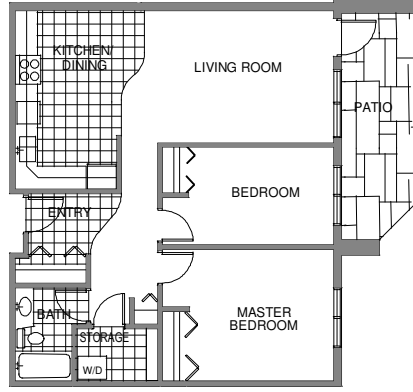
PHASE 2 TYPE: A 932 SQ. FT.
